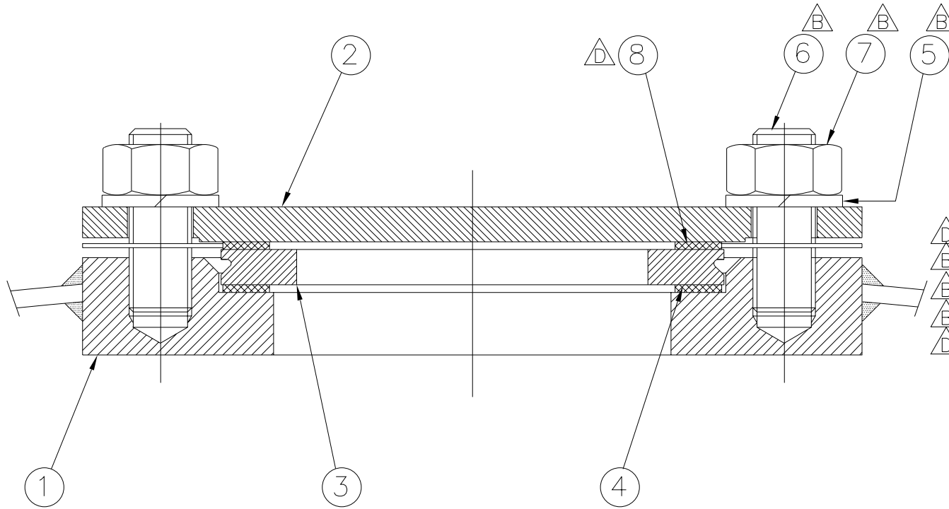
SECTION THROUGH TOP DISCHARGE ASSEMBLY
